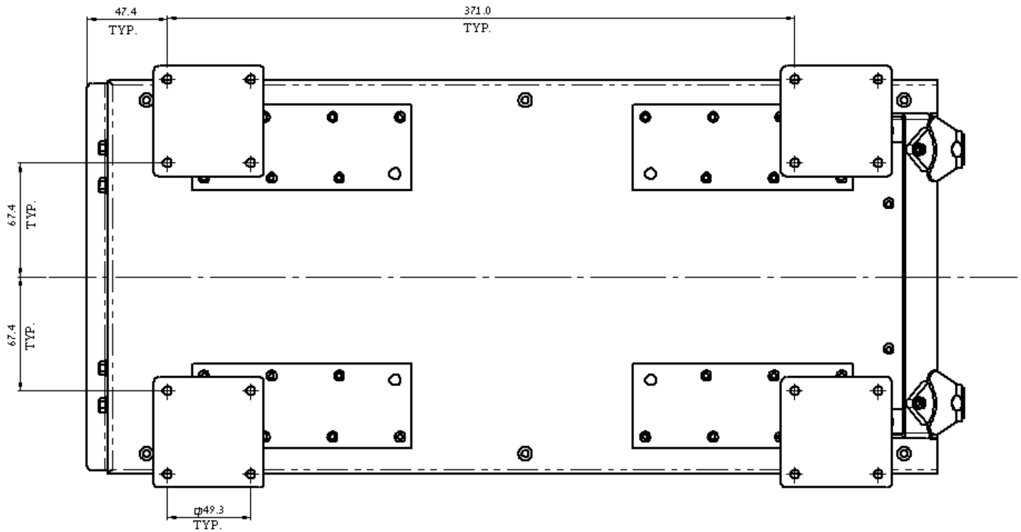
BOTTOM VIEW WITH SHOCK MOUNTS FM26
